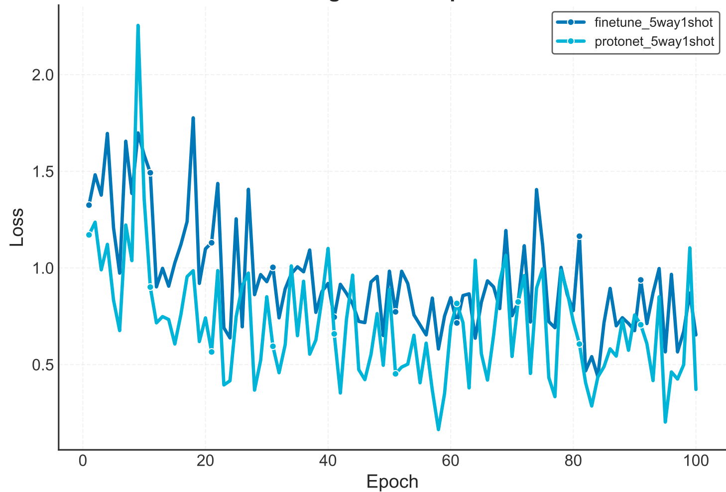
Training Loss Comparison
